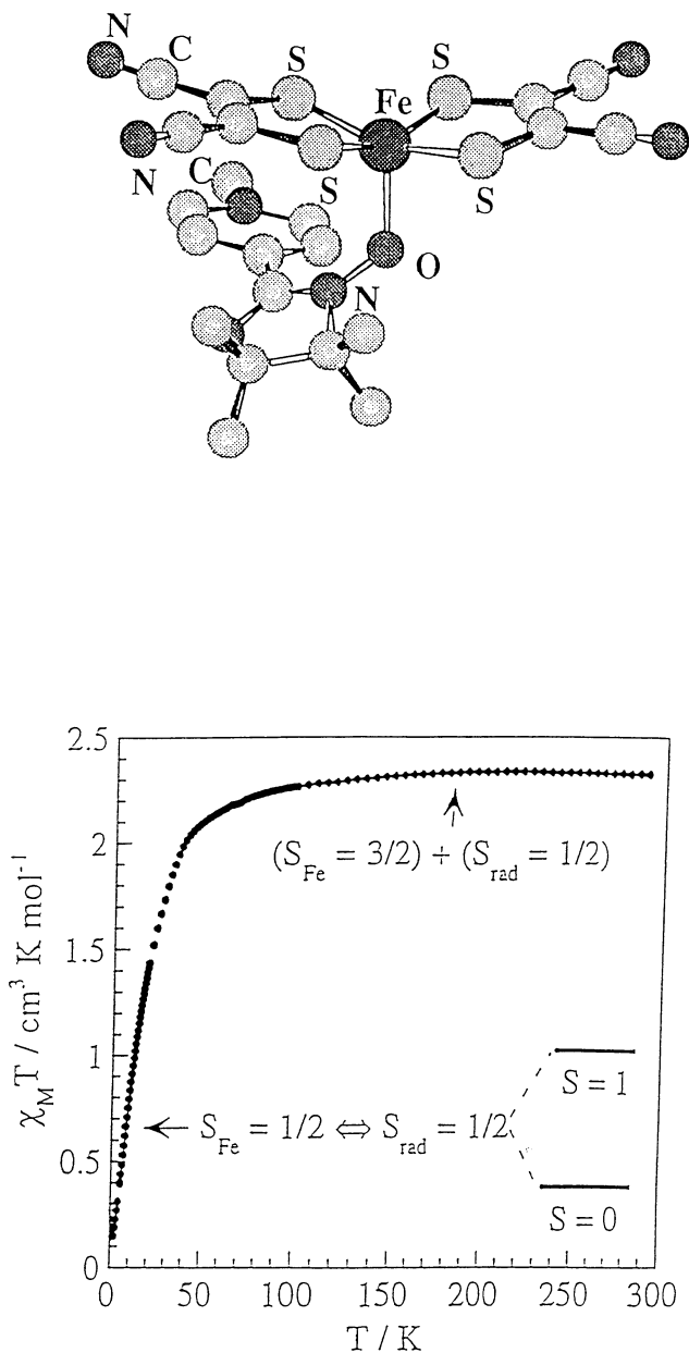
Fig. 17. Molecular structure and temperature dependence of the \chi_M T product for \text{Fe(mnt)}_2\text{-rad} .
